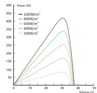
Power-Voltage Curve(425W)
